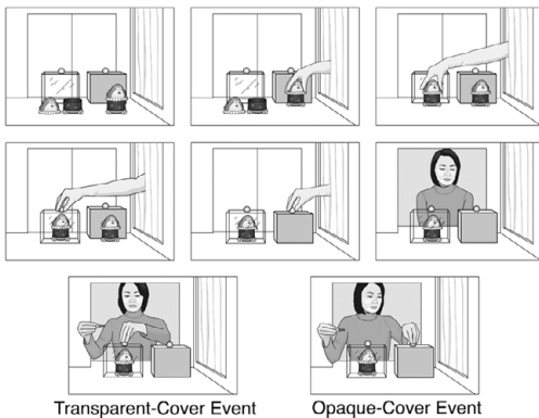
Transparent-Cover Event
